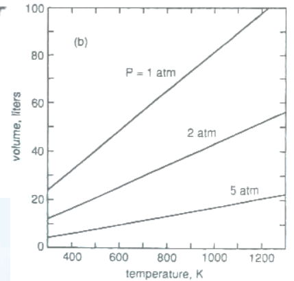
Figure 1.3 (a) The variations, with pressure, of the volume of 1 mole of ideal gas 300 and 1000 K. (b) The variations, with temperature, of the volume of 1 mole of ideal gas at 1, 2, and 5 atm.
